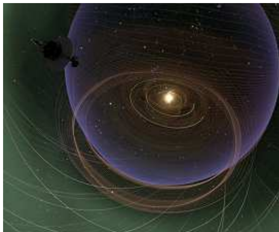
Voyager flies through the outer bounds of the heliosphere en route to interstellar space. A strong magnetic field reported by Opher et al in the Dec. 24, 2009, issue of Nature is delineated in yellow. Image copyright 2009, The American Museum of Natural History.
