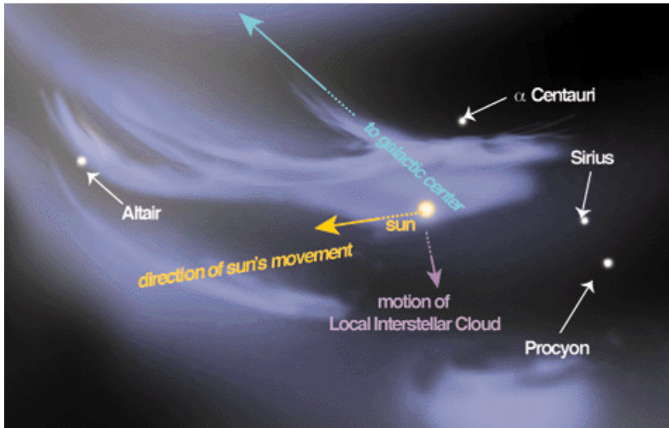
Above: An artist's concept of the Local Interstellar Cloud, also known as the "Local Fluff." Credit: Linda Huff (American Scientist) and Priscilla Frisch (University of Chicago) - http://antwrp.gsfc.nasa.gov/apod/ap020210.html
